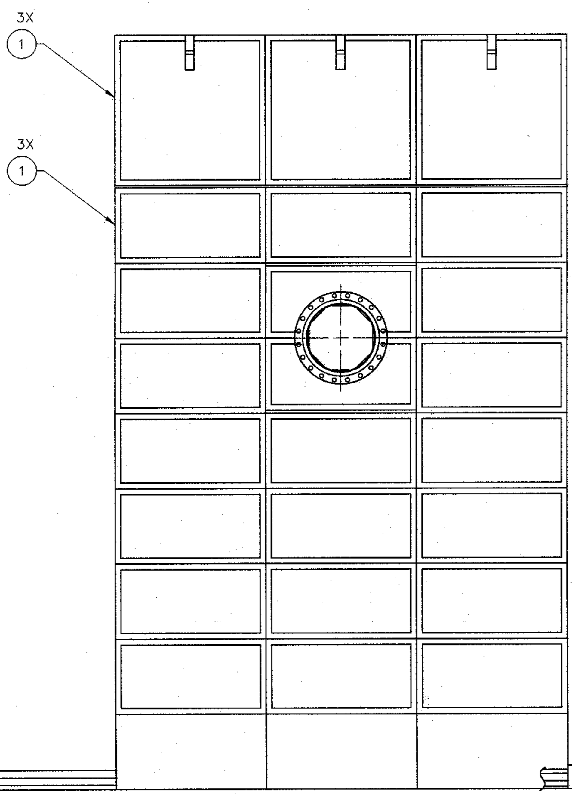
INSTALLATION STEP 3 (SHIELD BLOCKS, STEEL PLATE)
