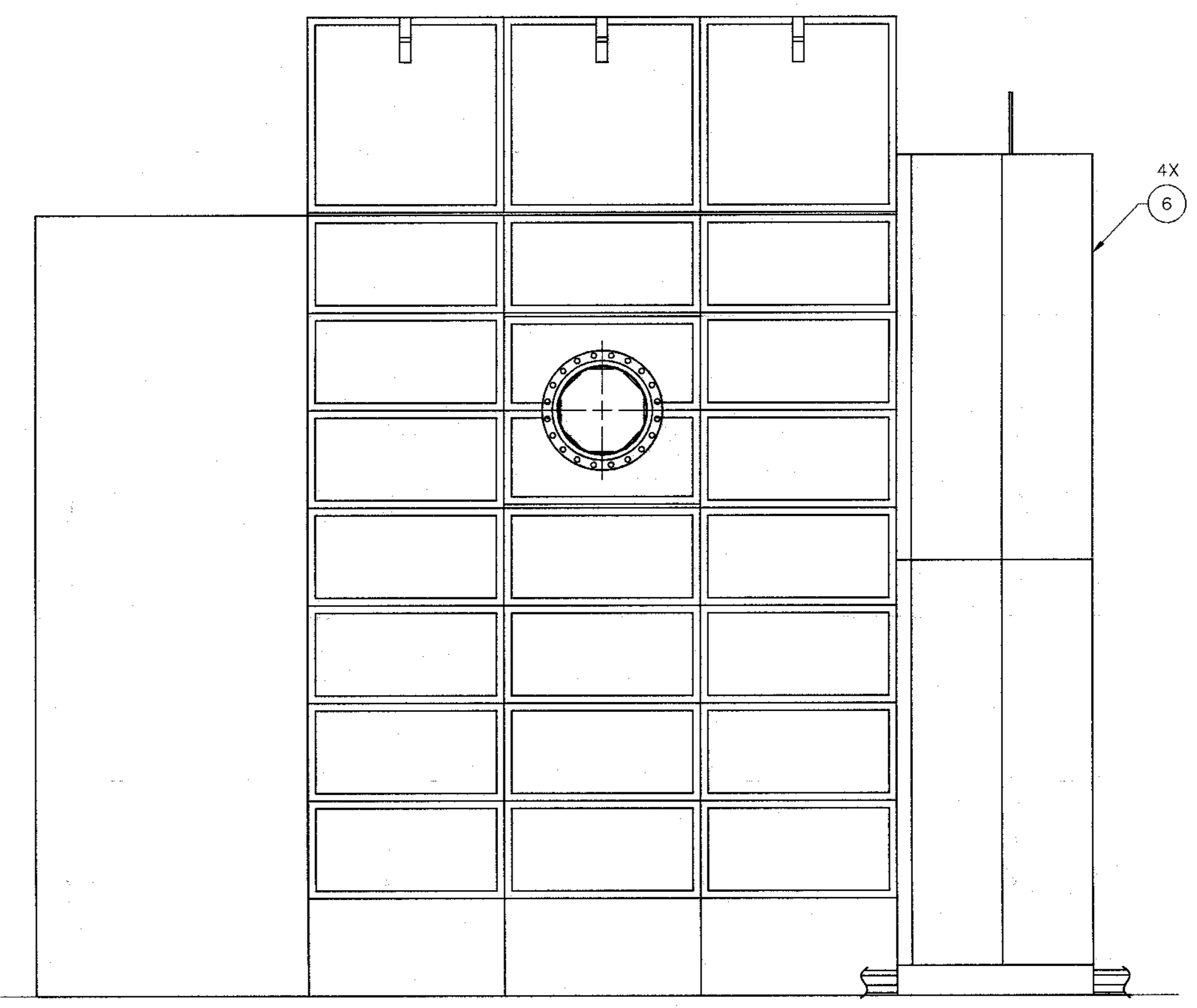
INSTALLATION STEP 4 (LEAD SHEET, STEEL PLATES)
