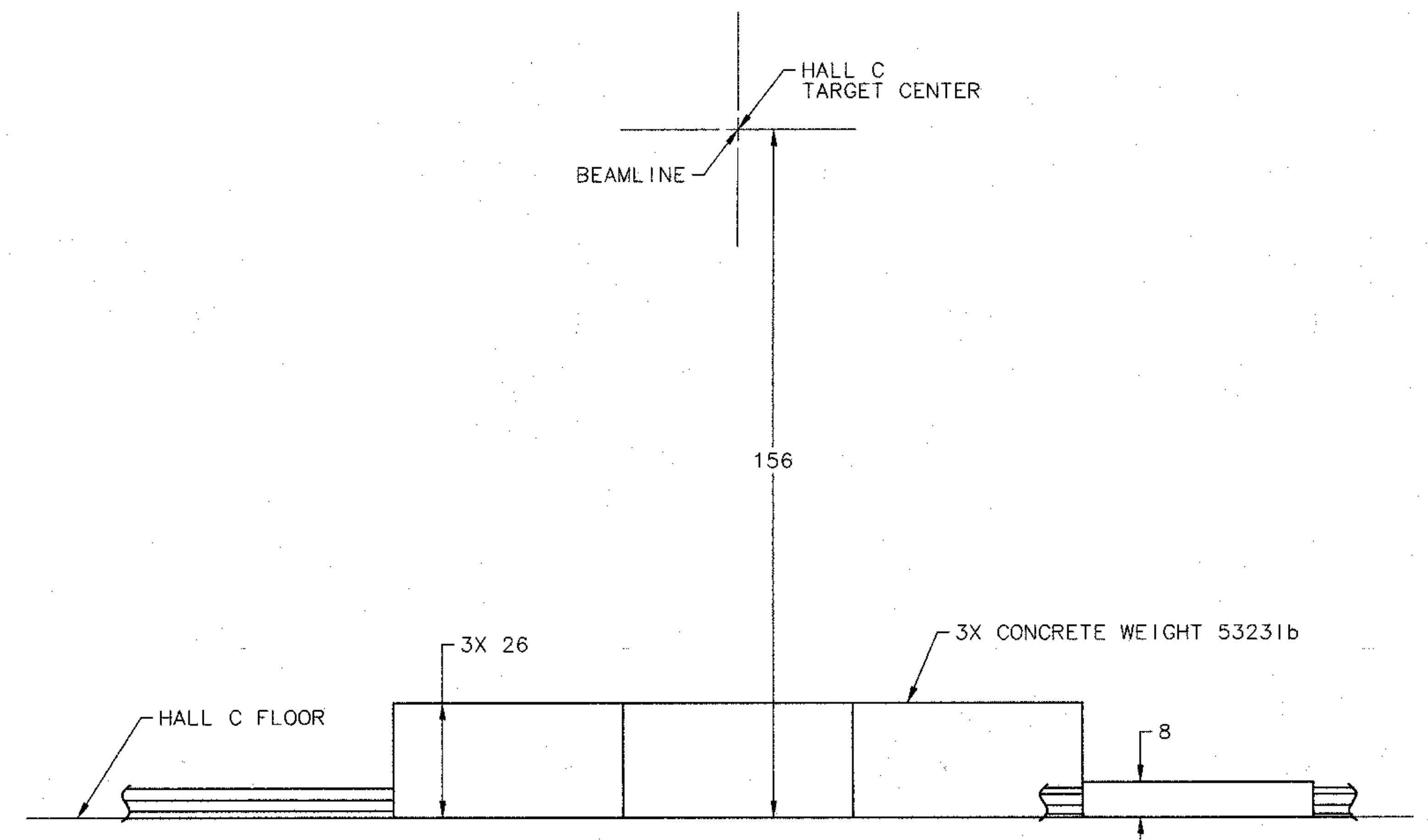
INSTALLATION STEP 1 (CONCRETE PADS)
