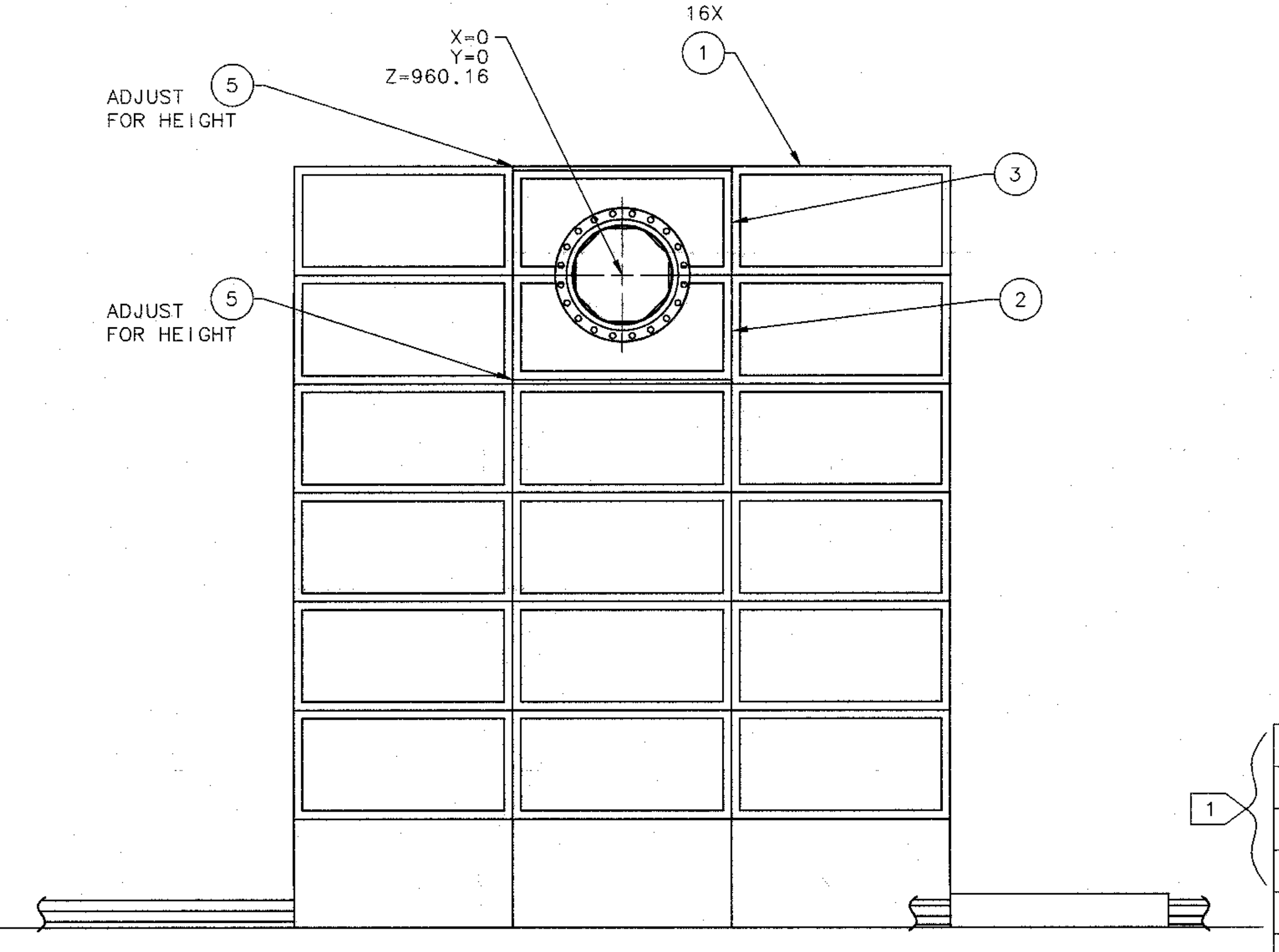
INSTALLATION STEP 2 (SHIELD BLOCKS, STEEL SHIMS, BEAMPIPE)
